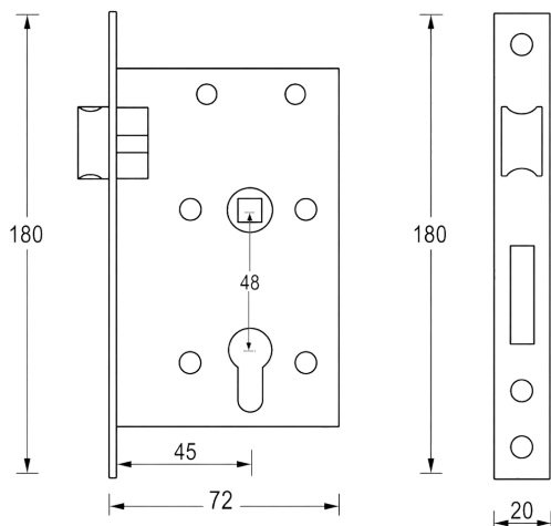
45mm Backset
